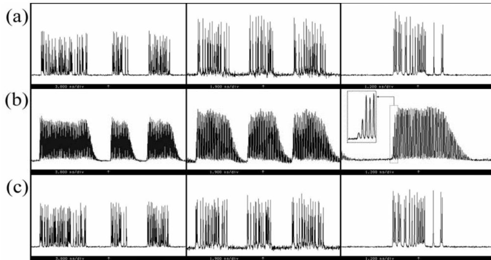
Fig. 2. Pulse traces. First column: synchronous operation (time scale 3.8 ns/div), second column: asynchronous operation (time scale 1.9 ns/div), third column: individual packet (time scale 1.2 ns/div). (a): input signal, (b): recovered clock, (c): recovered signal. The inset of the clock packet in (b) shows the rise-time at a timebase of 200 ps/div
