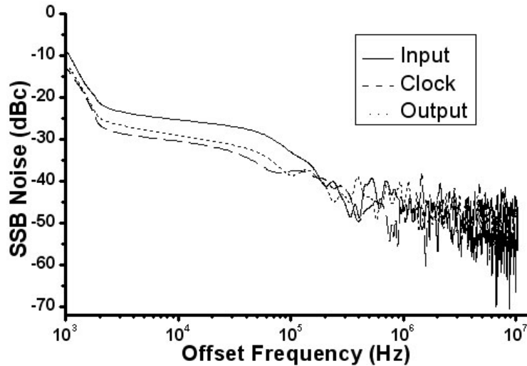
Fig. 4. SSB noise spectra of the input, clock and recovered signal.
