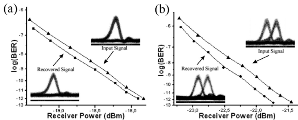
Fig. 3. BER measurements and acquired eye diagrams for the two data patterns used.
