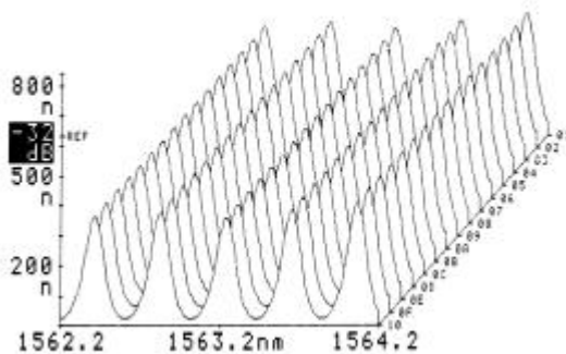
Figure 5: Output time evolution over 90 minutes.
