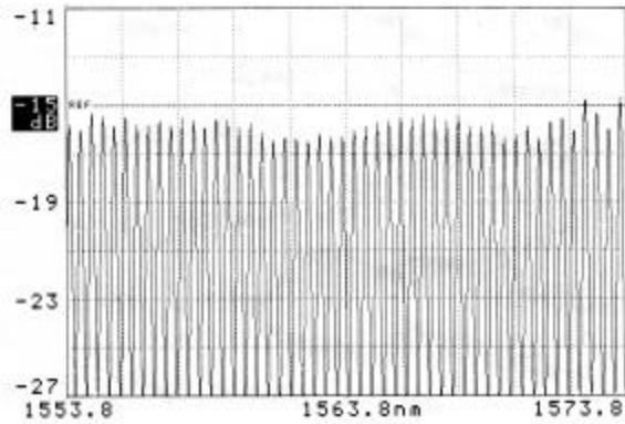
Figure 3: Optical spectrum of the multi-wavelength laser (sweep width 2 nm/div).
