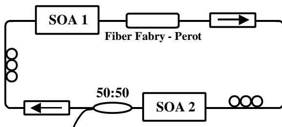
Figure 1: Experimental layout of the multi-wavelength ring laser.
