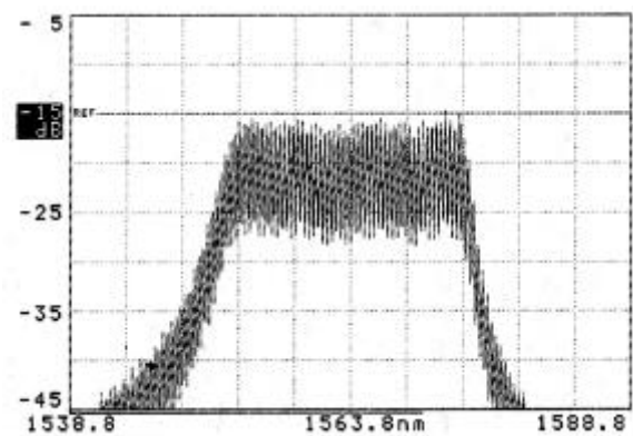
Figure 2: Optical spectrum of the multi-wavelength laser (sweep width 5 nm/div).
