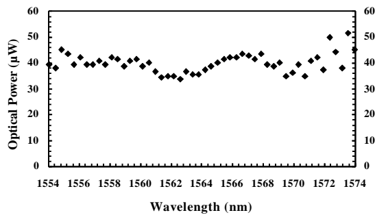
Figure 4: Power distribution for output wavelengths.
